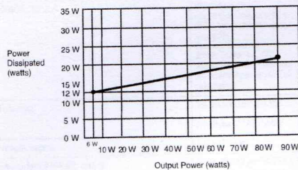
1768-PB3 Power Dissipation
