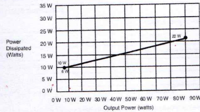
1768-PB3 Power Dissipation
