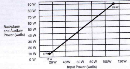
1768-PB3 Input Power Requirements
