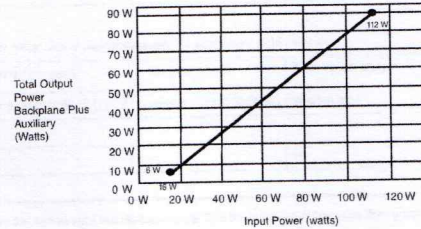
1768-PB3 Input Power Requirements
